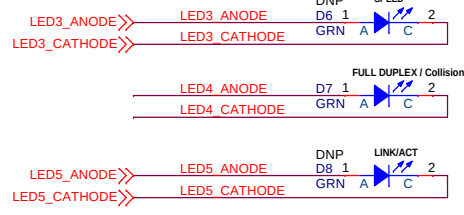
Port 2 LEDs
