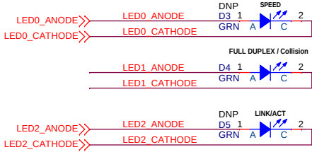
Port 1 LEDs
