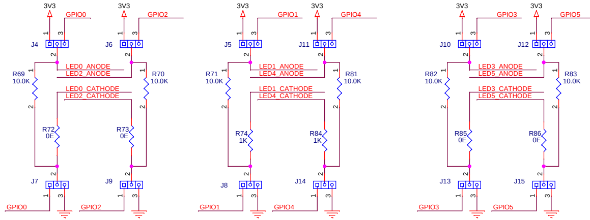
Port 1 LEDs
